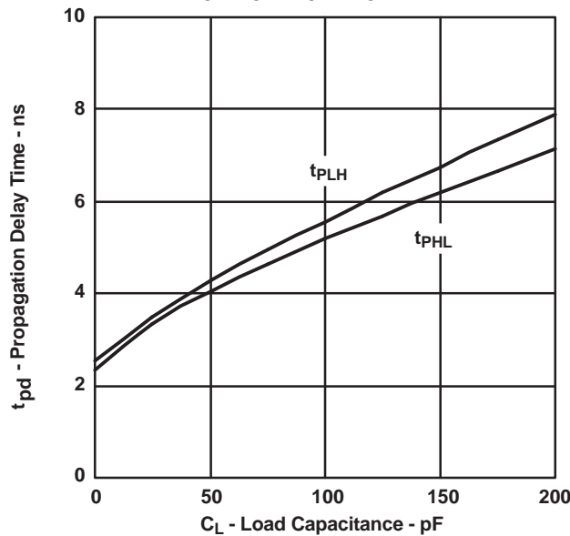
TYPICAL PROPAGATION DELAY vs LOAD CAPACITANCE
